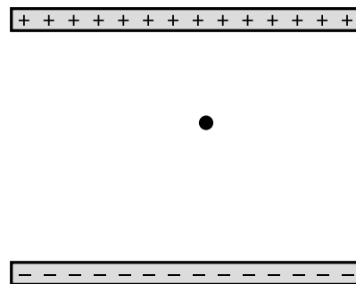
g / A simplified diagram of Millikan's apparatus.
